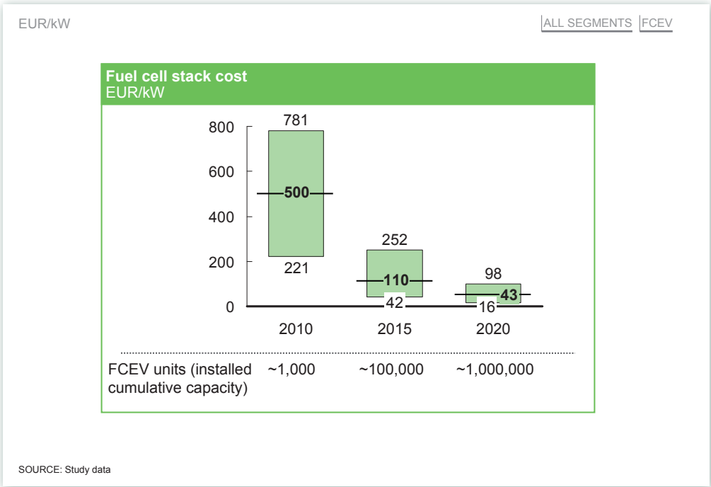
Exhibit 54: The cost of the fuel cell stack, based on data submitted by participating car manufacturers and suppliers
